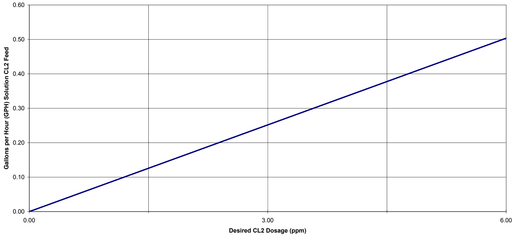
Well 4 Chlorinator Disinfection with Sodium Hypochlorite 25.00% Solution @ 350 gpm
