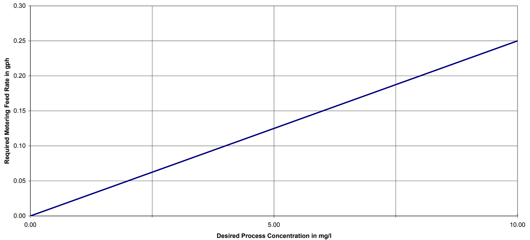
Alum (Aluminum Sulphate) Process Dosage Rates for Treatment Plant 100 gpm Process Flow
